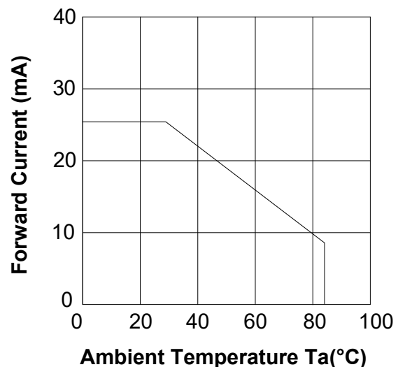
Maximum Forward Current vs. Ambient Temp.
