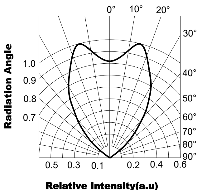
Directivity (Ta=25°C)
