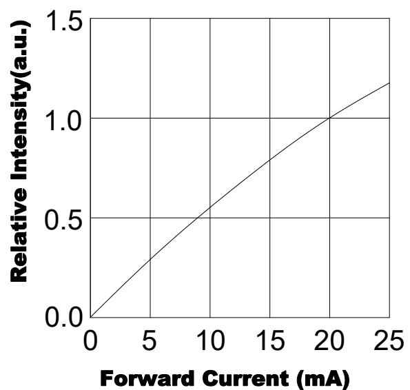
Relative Intensity vs. Forward Current (Ta=25°C)
