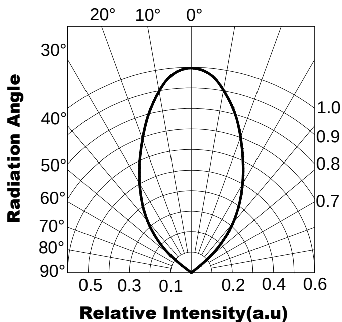
Fig.6 Relative Radiant Intensity vs. Angular Displacement
