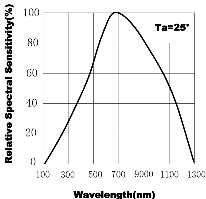
Fig.2 Spectral Sensitivity
